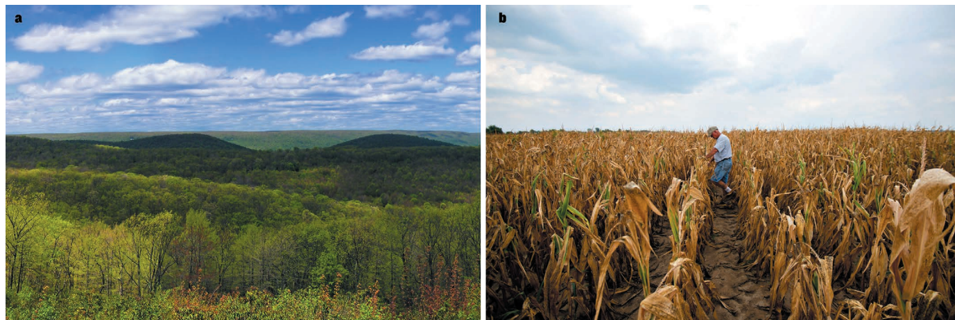
Figure 1 | Seasonal and regional variations of carbon uptake in the continental United States. a, Eastern temperate forests grew vigorously during the warm spring of 2012, and took up more carbon than normal for this season. b, The subsequent hot, dry summer caused crops to fail in the Great Plains, and carbon uptake in this region was lower than normal. Wolf et al. 2 report that the spring carbon uptake offset the summer carbon losses across the continental United States.
